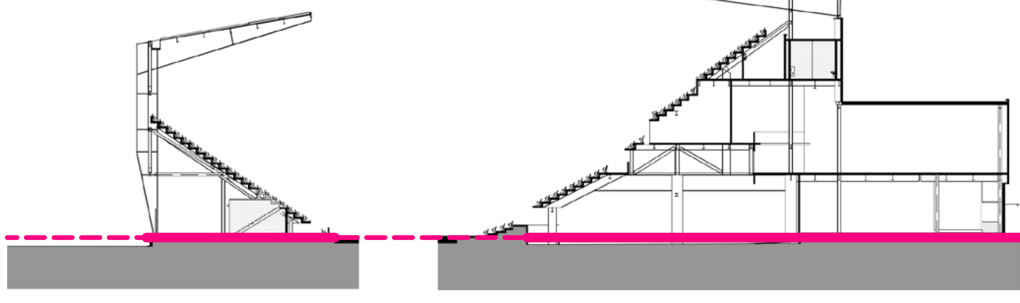
WEST SECTION
