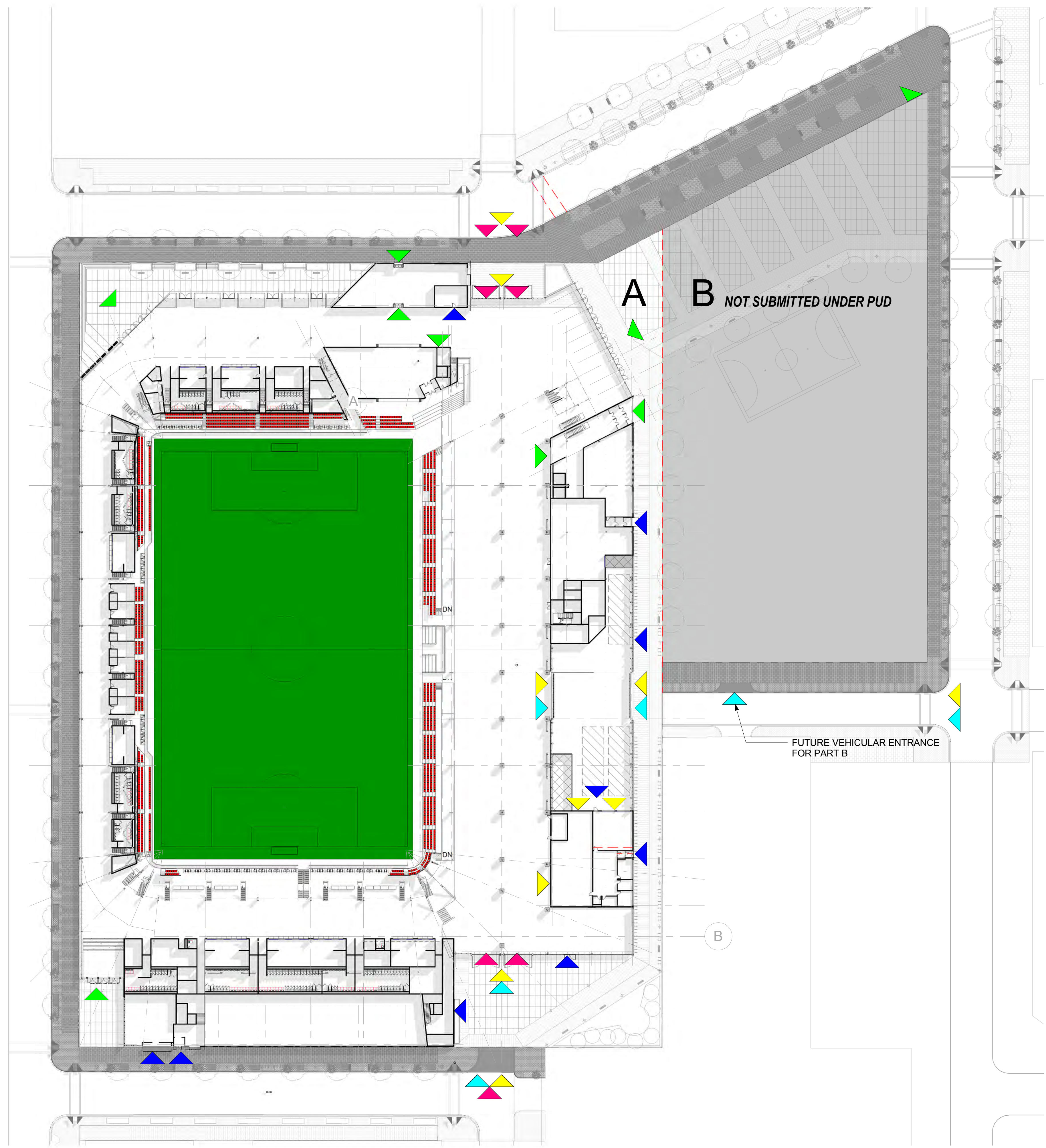
1 CIRCULATION AND LOADING PLAN 1" = 50'-0"
