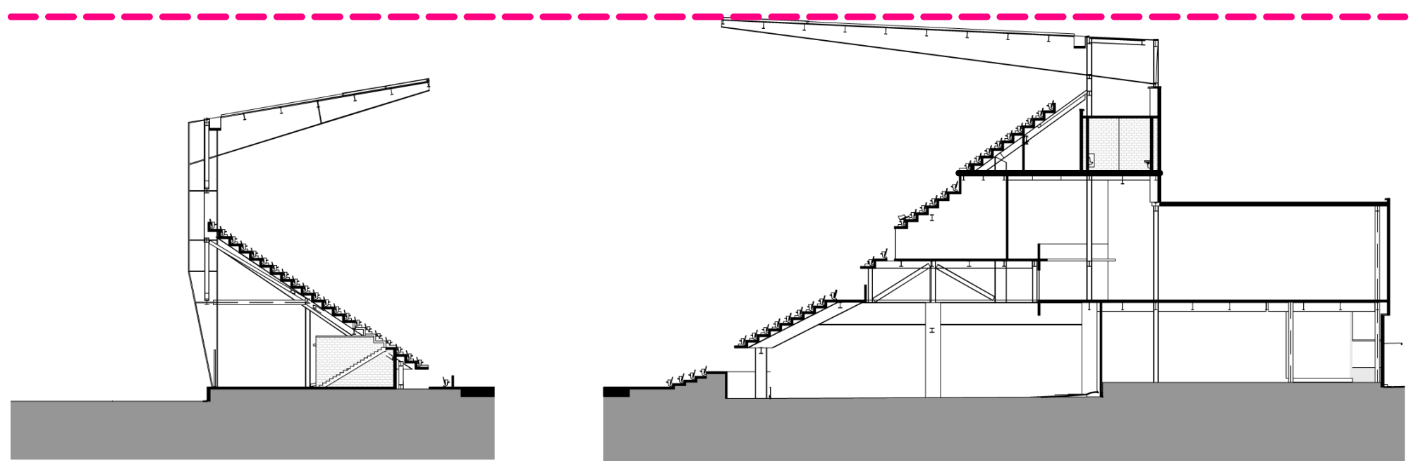
WEST SECTION
