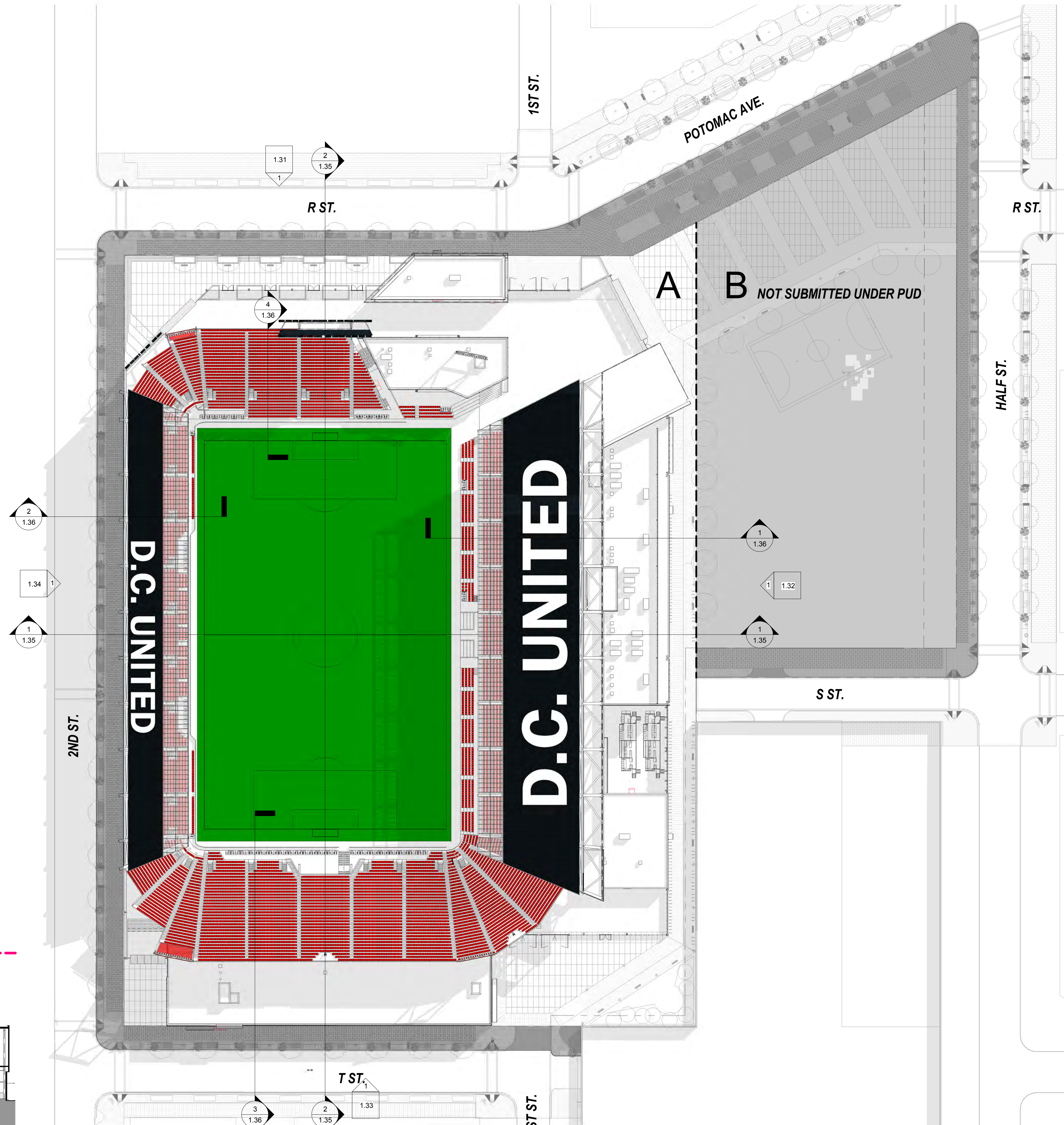
1 ROOF PLAN 1" = 50'-0"
